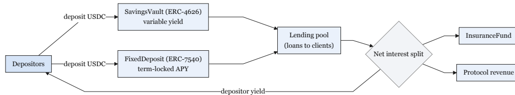
Figure 4.11: Savings vault.
