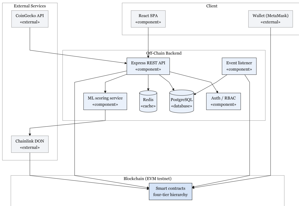
Figure 4.2: Component diagram.
