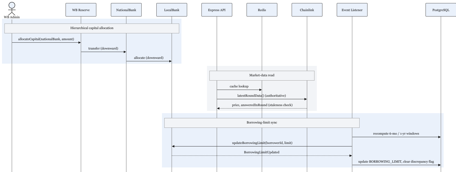
Figure 4.22: Hierarchical banking and data sync.
