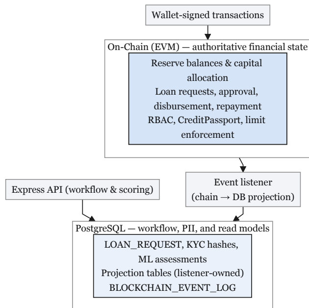
Figure 4.7: Financial data lifecycle.
