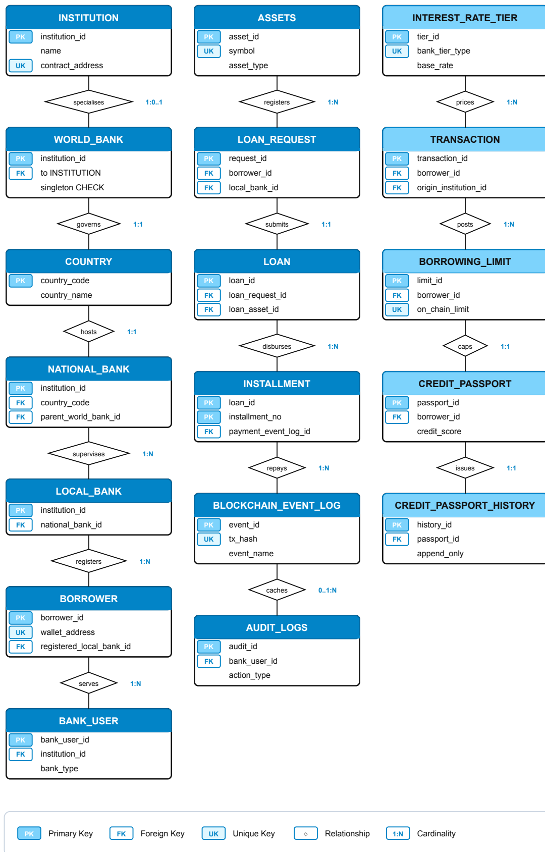
Figure A.1: Full relational ERD (sheet 1 of 2).
