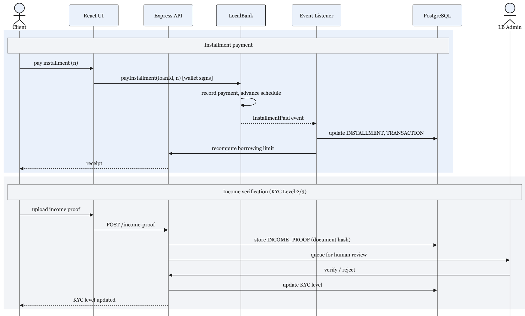
Figure 4.21: Installment and income verification.
