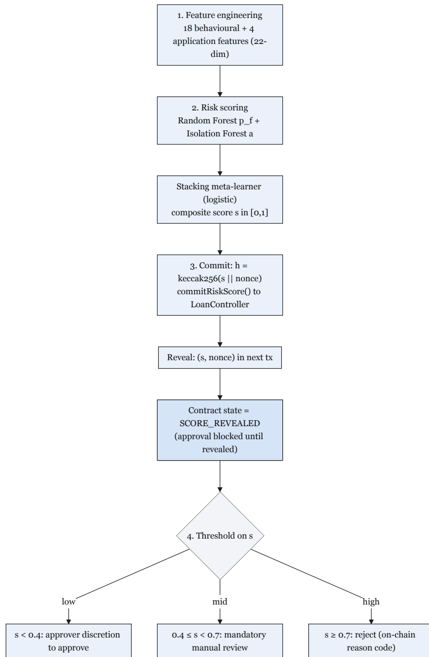
Figure 4.30: ML oracle commit–reveal.
