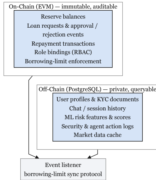
Figure 4.6: Data partitioning diagram.
