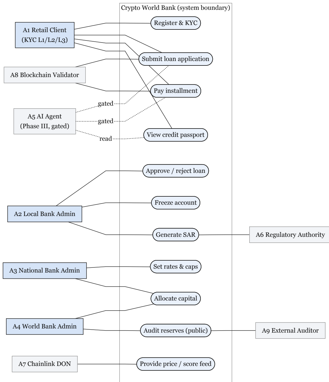
Figure 4.14: Use-case diagram.
