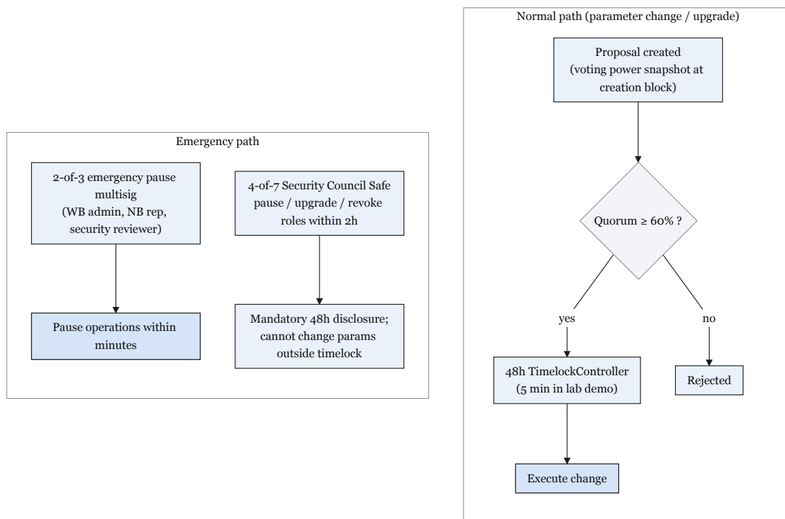
Figure 4.27: Governance dual-path.
