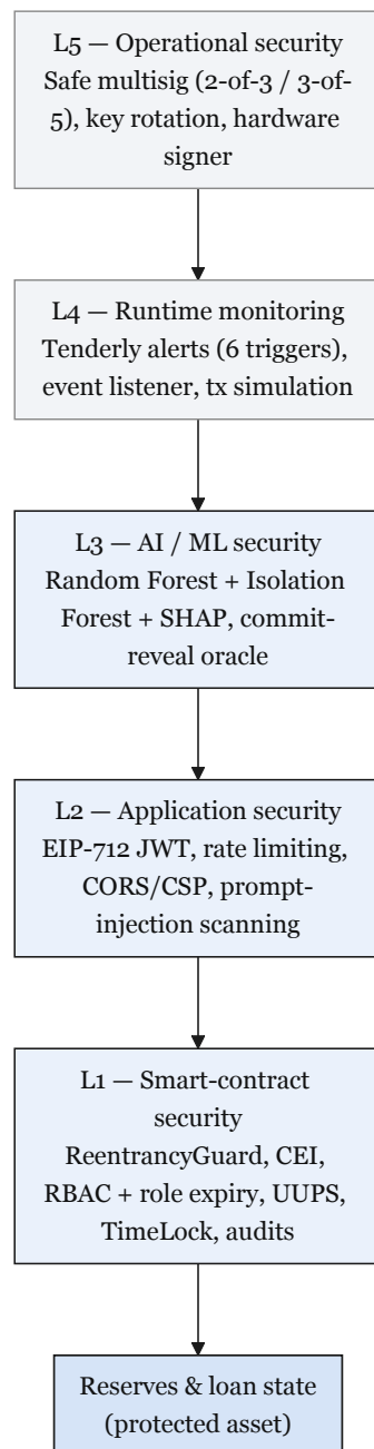
Figure 4.29: Defense-in-depth architecture.
