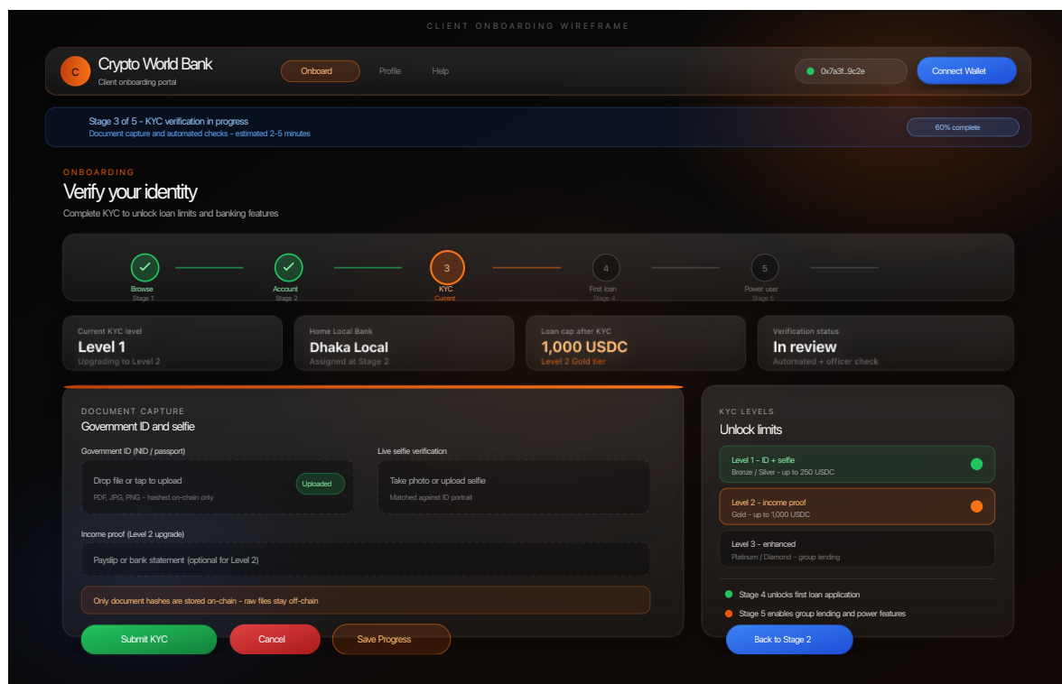
Figure C.3: Onboarding wireframe.
