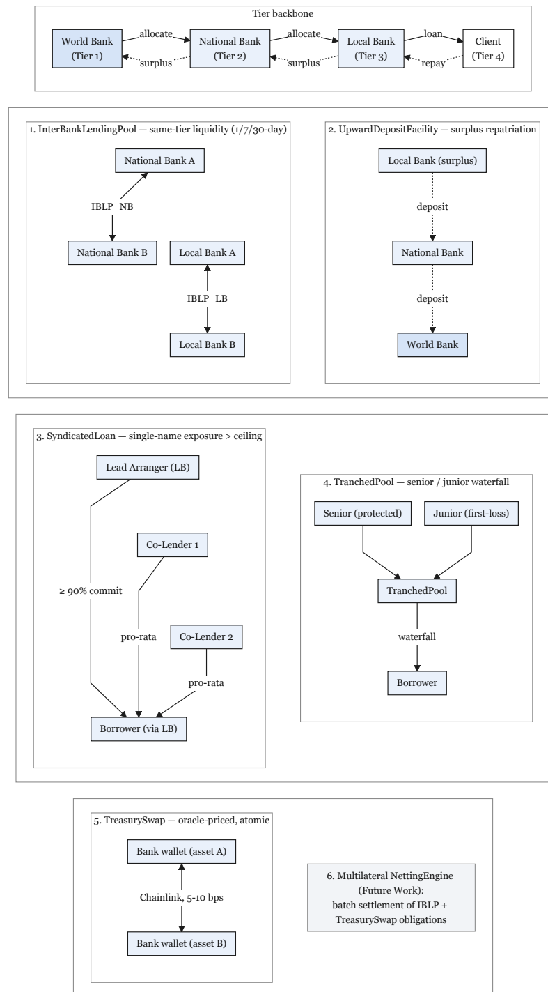
Figure 4.13: Multi-entity operations.
