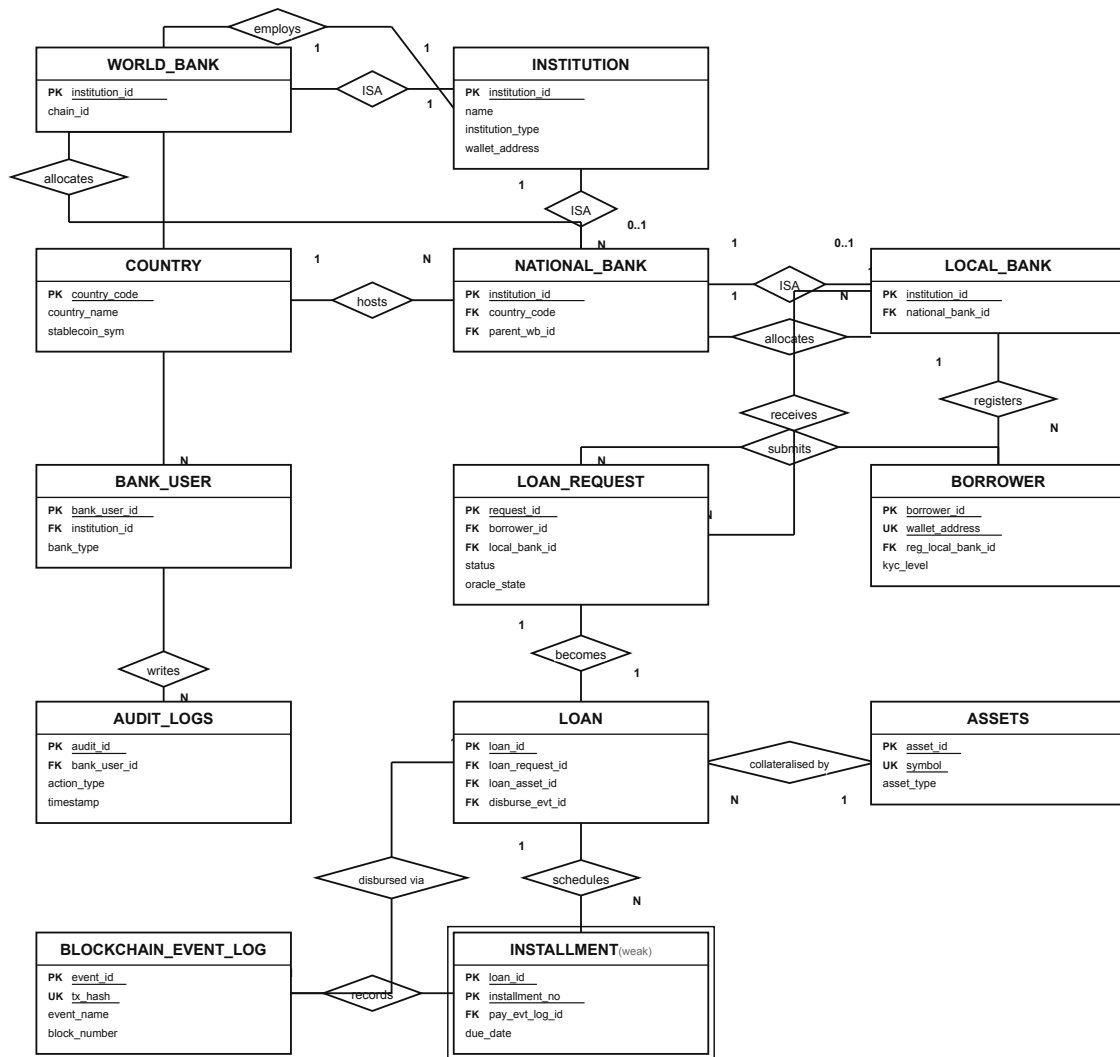
Figure 4.5: Core entity graph.
