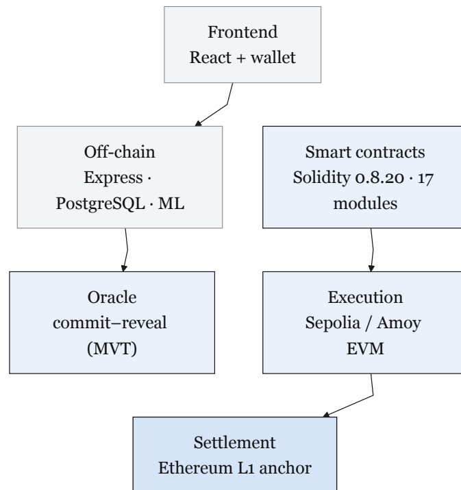
Figure 4.3: Blockchain stack.
