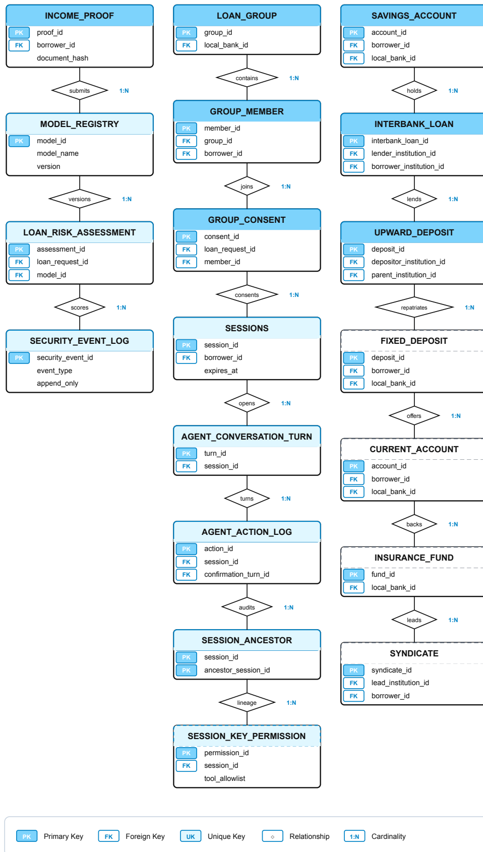
Figure A.2: Full relational ERD (sheet 2 of 2).
